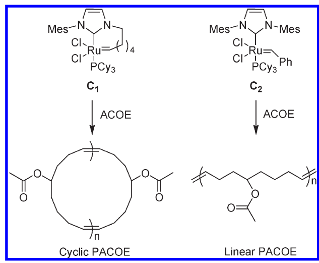
Scheme 1. Structures of the Cyclic REMP Catalyst C1 and Olefin Metathesis Catalyst C2, and the Resultant Cyclic PACOE and Linear PACOE
